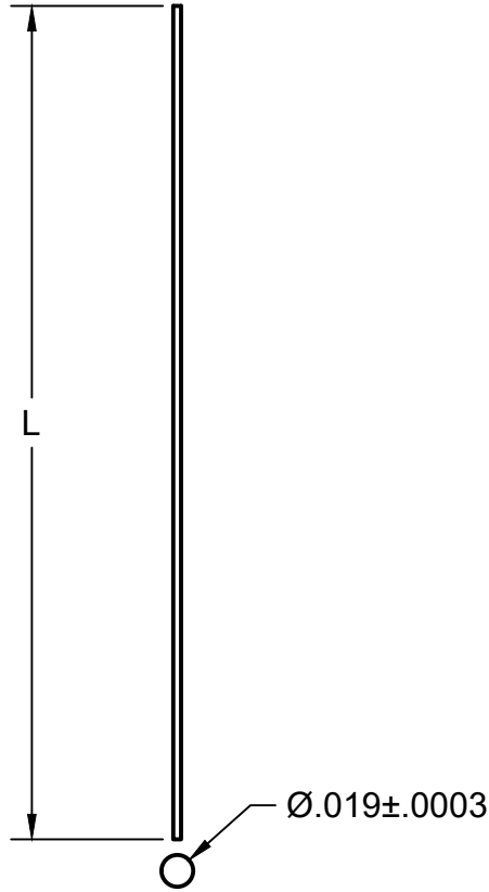
DETAIL A SCALE 8:1
