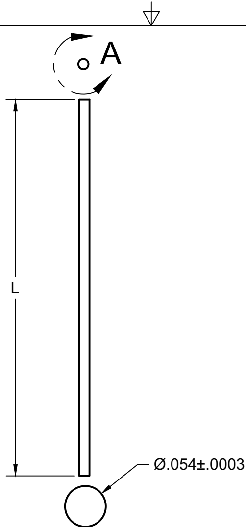
DETAIL A SCALE 8:1
