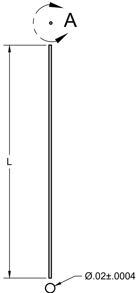
DETAIL A SCALE 8:1
