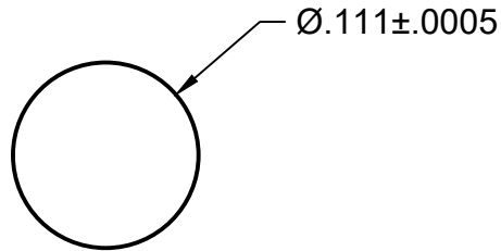
DETAIL A SCALE 8:1
